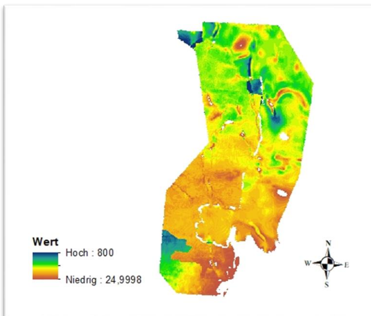
Figure 12: range of thickness for “nls3d_04_near_base_cenozoic_thickness_3034”.
