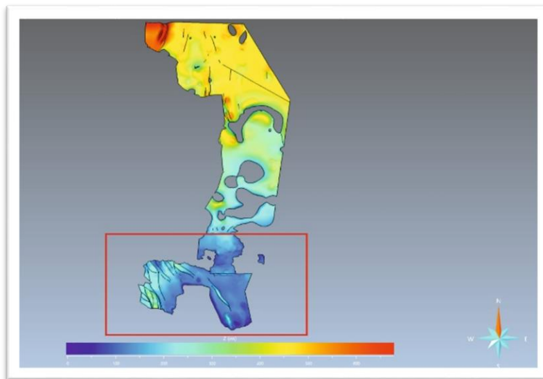
Figure 5: Remodeling of Near Base Lower/Middle Miocene and Base Rupel in Lower Saxony. The red rectangle shows the area that was remodeled with SubsurfaceViewer.
