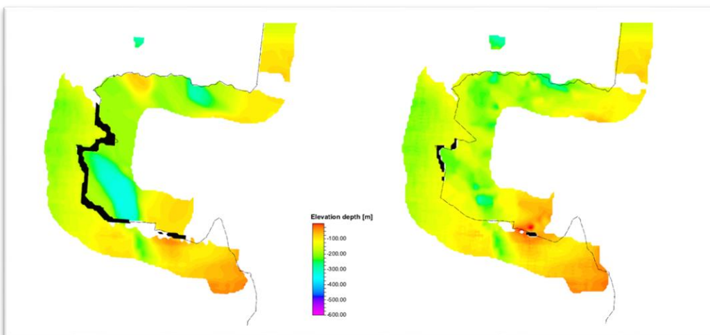
Figure 7: Comparison of the German models with their depth position; left: 05_tolm-tolo from GTA3D; right: remodeled “Nordhorn area”. Black spots show areas of no harmonization.
