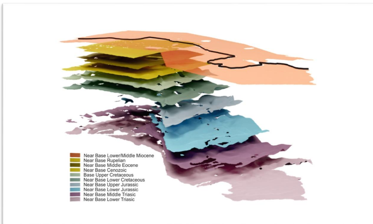
Figure 2: NLS3D – 3D view into the 3D model
