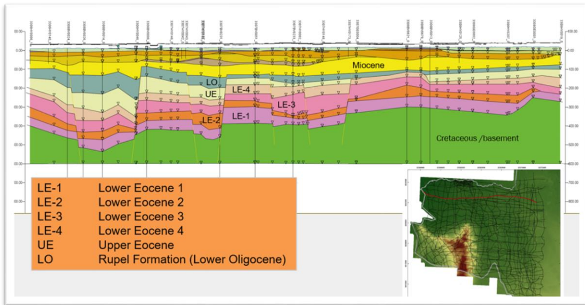
Figure 6: West-east cross-section, showing remodeled horizons LO= Base Rupel and Miocene = Base Lower/Middle Miocene in the “Nordhorn area”.
