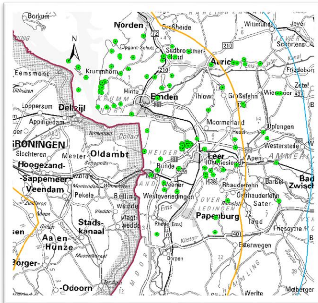
Figure 13: Wells with lithostratigraphic description of Brüssel Sand in Lower Saxony.
