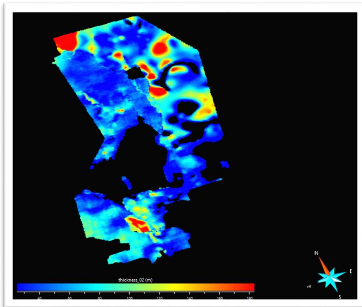
Figure 10: range of thickness for “nls3d_v2_02_base_rupelian_thickness_3034”.
