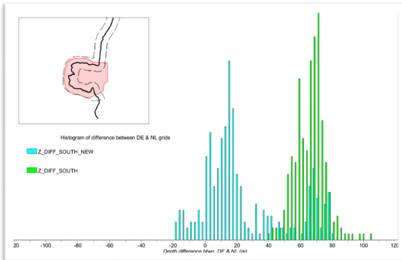
Figure 8: Comparison of the histograms of the depth differences between DE and NL for the remodelled “Nordhorn area” (blue) and the GTA3D (green).
