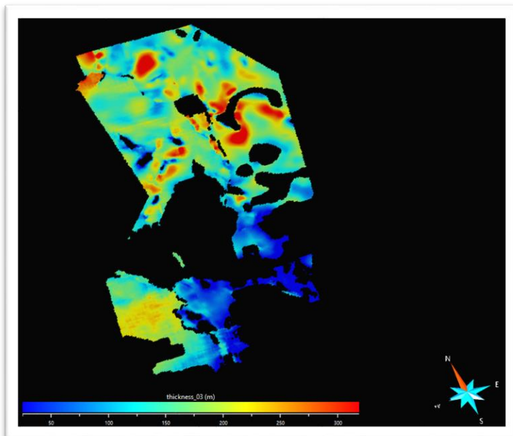
Figure 11: range of thickness for “nls3d_v2_02_base_rupelian_thickness_3034”.
