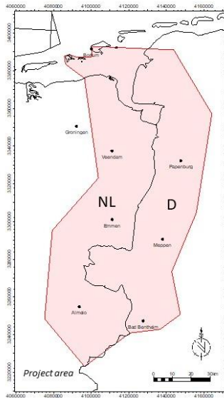
Figure 1: Pilot area of WP1, showing the extent of the harmonized 3D model NLS3D. Also the national border is shown, where the harmonization of existing models was realized.
