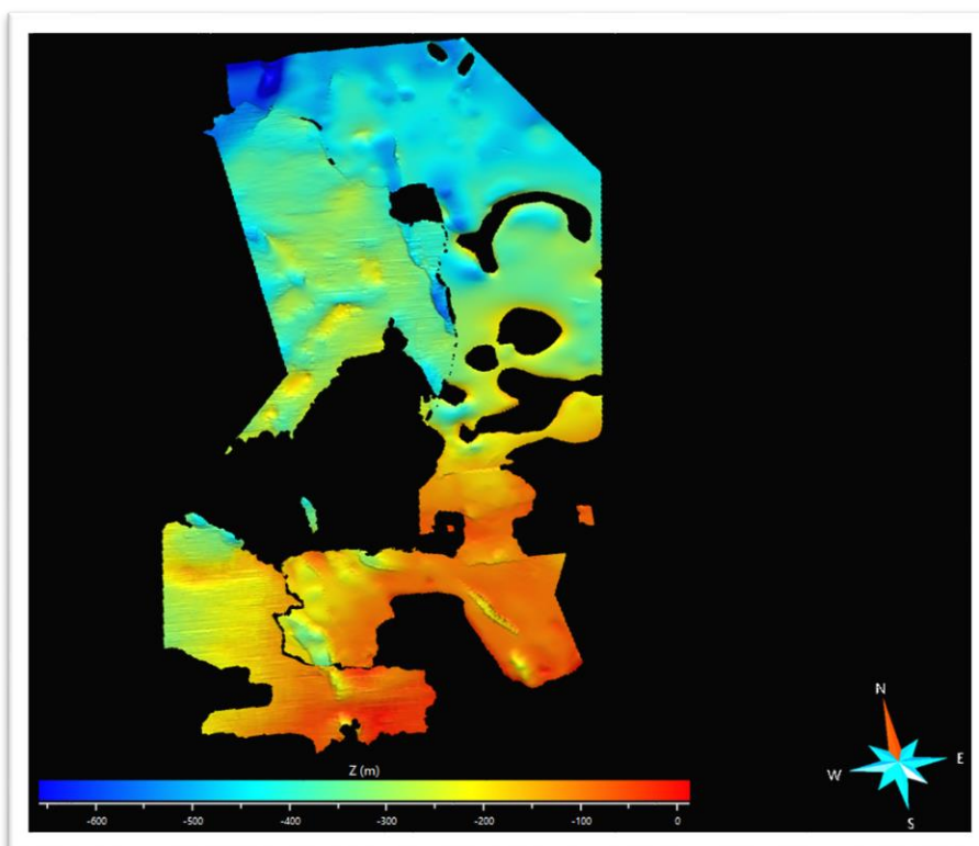
Figure 14: Decision support map showing distribution and depth of "Near Base Rupelian" (NLS3D).
